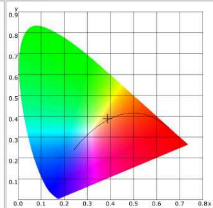
CIE1931
