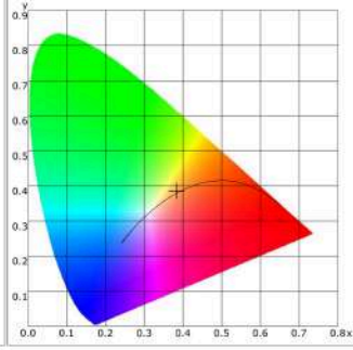
CIE1931
