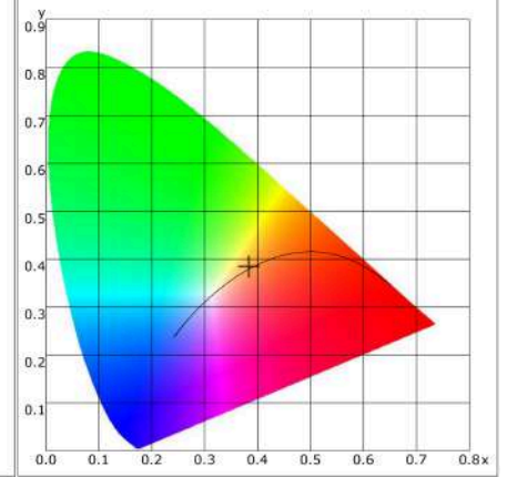
CIE1931
